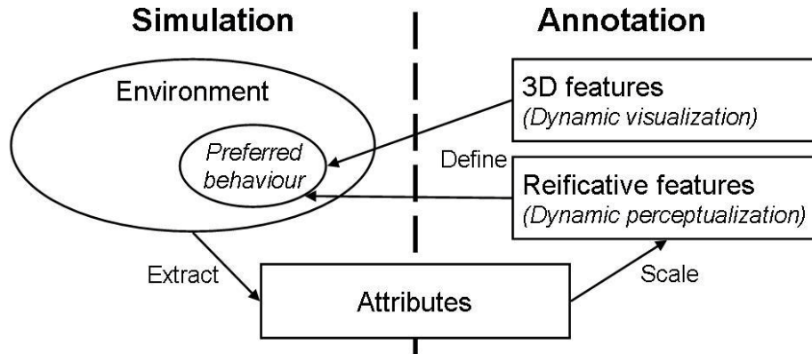
Fig. 1. Annotation of interactive simulation. Preferred behaviour of the simulated environment is annotated as 3D and reificative features . Reificative features facilitate understanding of complex concepts by highlighting the essential from the whole data. They can be perceptualized dynamically using any modality, whereas 3D features can only be visualized. Simulation's attributes act as scaling factors on the reificative features, for example that length of an incision made by a surgeon depends on the size of the limb. 3D features are naturally in right scale without any modifications.
